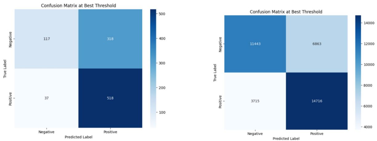
Fig. 9 Confusion matrices of similarity detection phase
