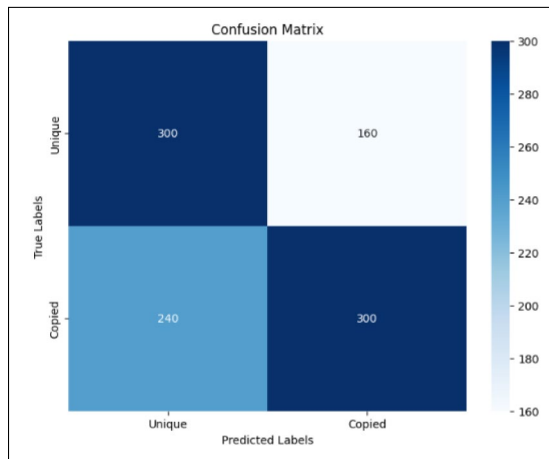
Fig. 10 Confusion matrix of online similarity detection method
